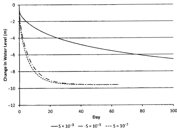
Figure 3. Sensitivity of the modeled head response to the storage coefficient used in the fractured shale for model layer 39 just above the shale.
