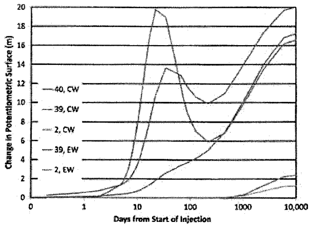
Figure 8. Simulated potentiometric surface changes for layers within the shale and sandstone. CW is center monitoring well and EW is east monitoring well, about 120 m from the centerline. Fault is included. The line for layer 2, CW plots beneath the line for layer 2, EW. K_{ss} = 0.01 m/d, K_{sh} = 0.001 m/d, S (fractured shale) = 0.001/m, S (ss) = 0.0001/m.
